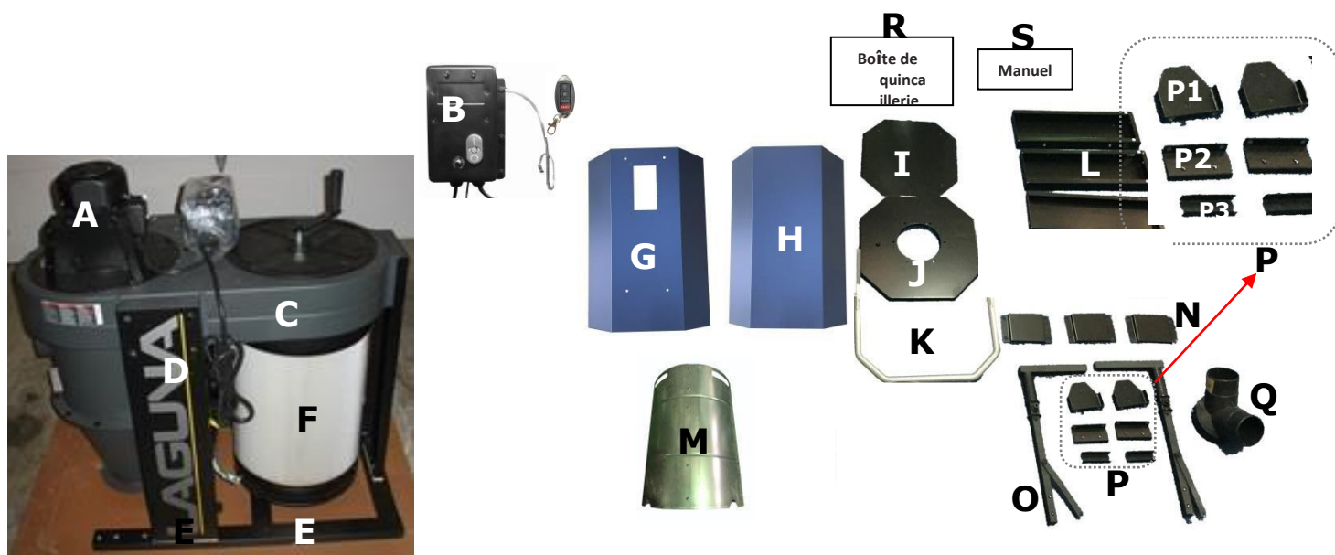
Figure 6 : Composants/Inventaire
