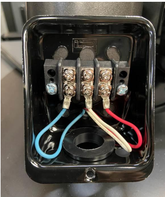
Figure 19: 220V Bottom Wiring in Junction Box Figure 20: 220V Top Wiring in Junction Box
