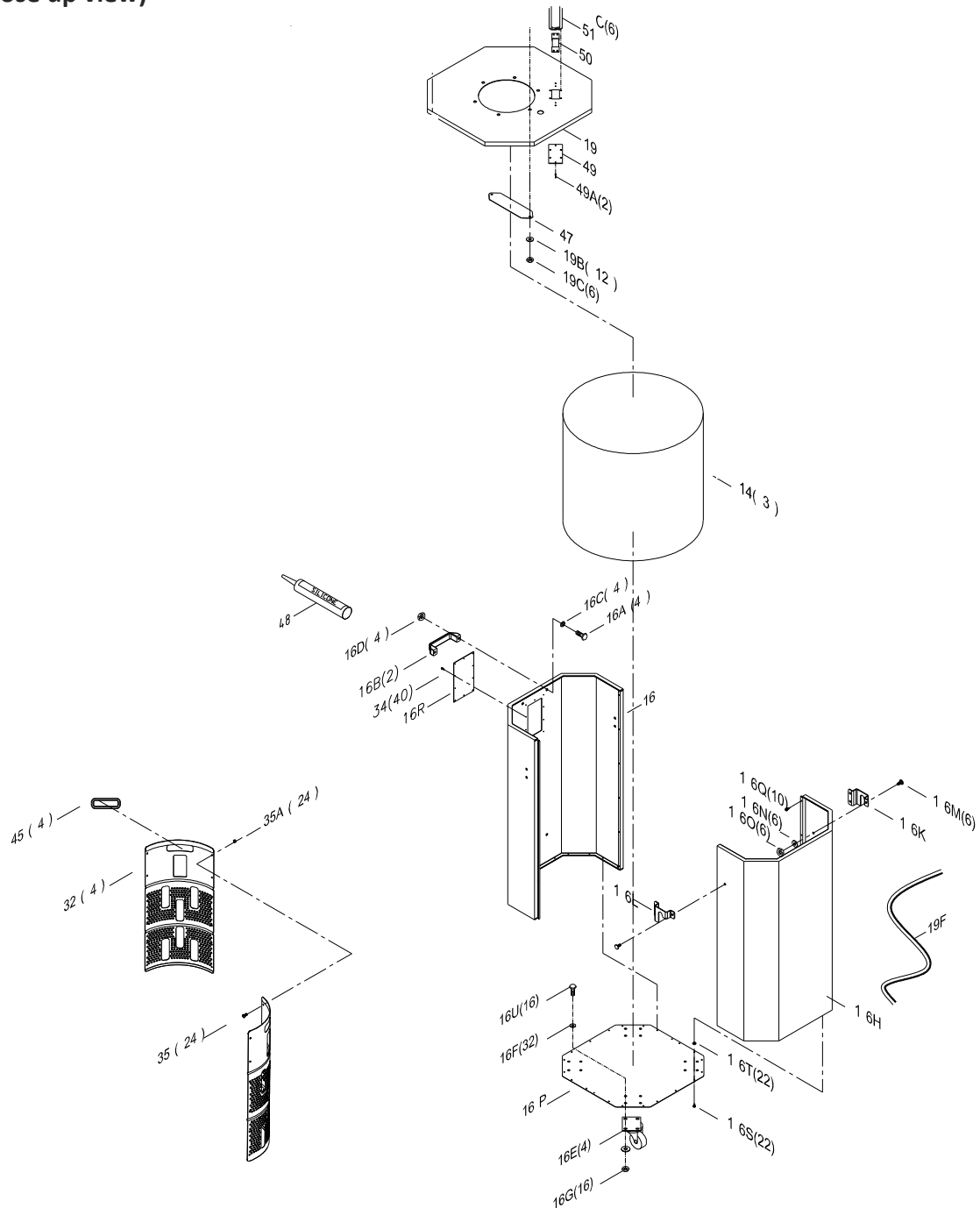
Figure 51: Barrel & insert
