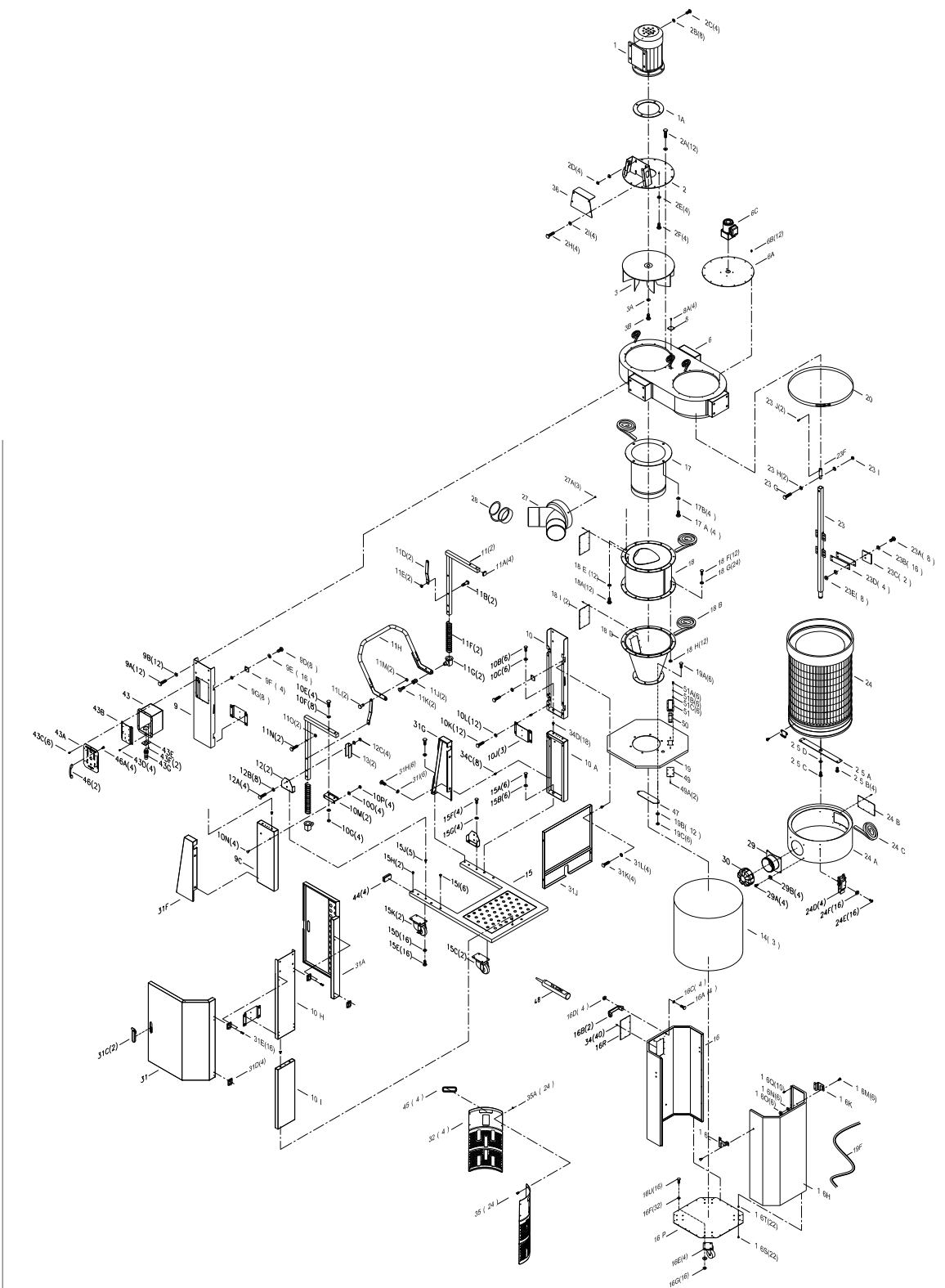
Figure 47: Main unit
