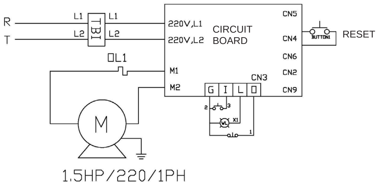
220V Power connections & wiring
